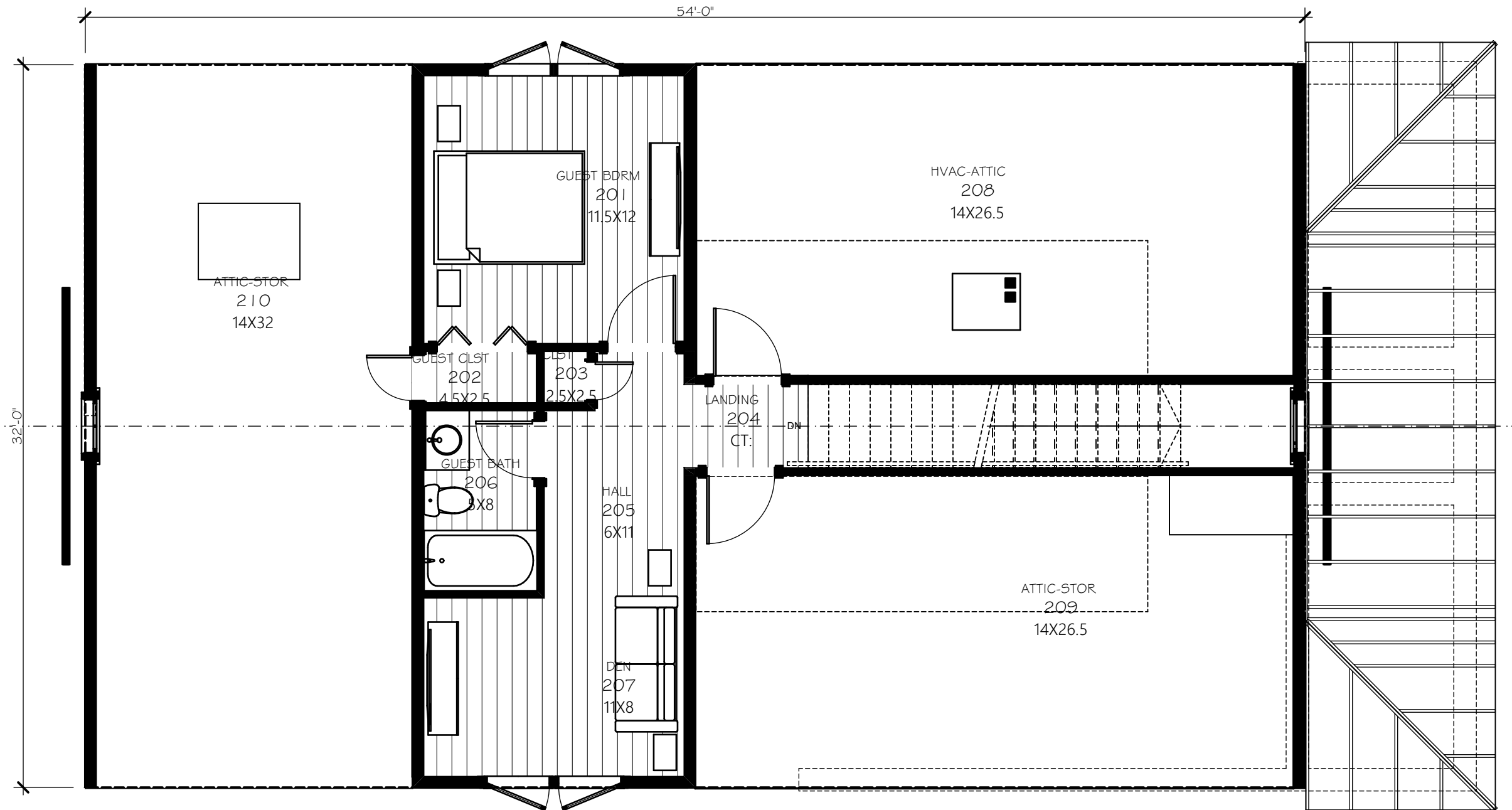
2nd FLOOR PLAN - CRAFTSMAN COTTAGE
